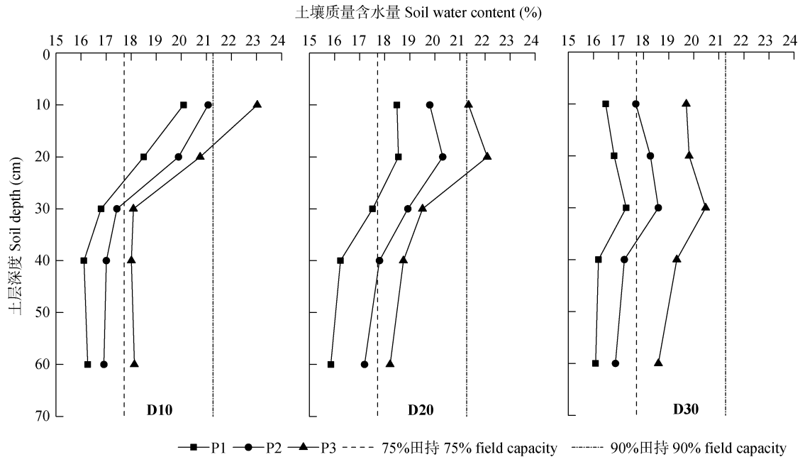
图 4 微润灌溉下不同微润管埋深和密度的番茄根区土壤 0~60 cm 土层含水量 Fig. 4 Changes of soil water contents in 0–60 cm soil layers of tomato root zone under different moistube depths and densities of moistub-irrigation
